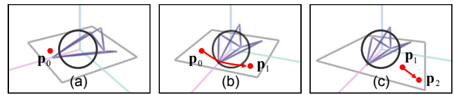
Figure 9: Space navigation: (a) initial state, (b) tumble (trackball), (c) dolly-zoom.
