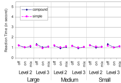
Figure 10. Reaction time by on-axis, off-axis, and mix-axes selections for both techniques, two and three level menus, and different input sizes.
